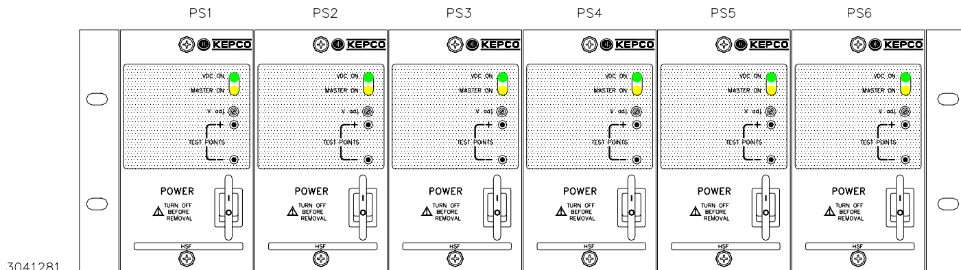
FIGURE 1. HSF-PFC 150 WATT POWER SUPPLIES (6) INSTALLED IN RA 19-6B RACK ADAPTER
