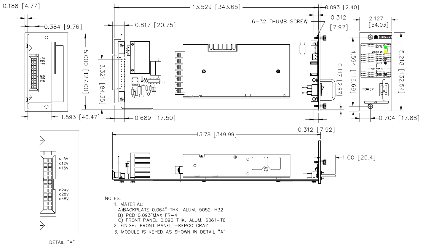
FIGURE 5. HSF-PFC 150W POWER SUPPLY OUTLINE DRAWING
